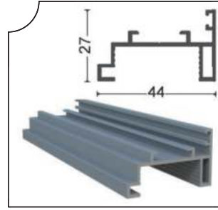
PRGLD-1006 Kollu Fıtil Karşılığı Contalı Esp.Handle Opposite Alm. Seal (With PVC Seal)
