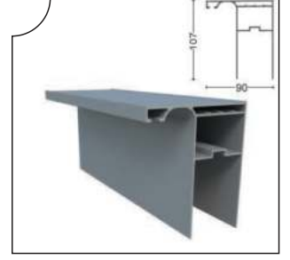
PRGLD-1003 Perdelik Ayak Profili Aluminum Curtain Profile
