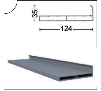
GYTN-1706 Alt Kasa Profili Lower Fram Profile
