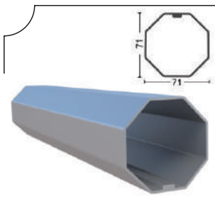
GYTN-2000 70'lik Sekizgen Boru Octogonal Aluminum Tubing
