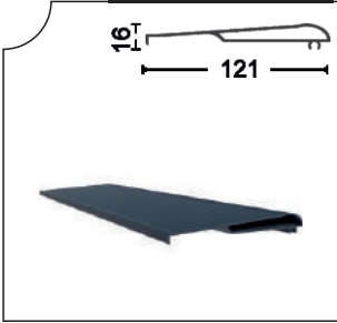
GYTN-1717 Hareketli Küpeşte Movable Handrail
