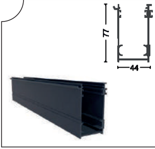
GYTN-1714 "U" Yan Dikme "U" Side Profile
