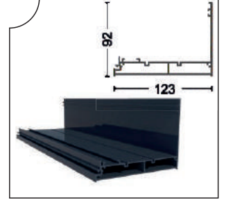
GYTN-1713 Yan Dikme Side Profile
