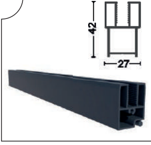
GYTN-1723 Alt-Üst Baza 8 mm Lower-Upper Base 8 mm Ağırlık/Weight 0.816 kg/m
