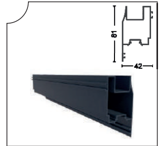
GYTN-1722 Ağır Kanat Isıcamlı Profile Of Insulated Opens
