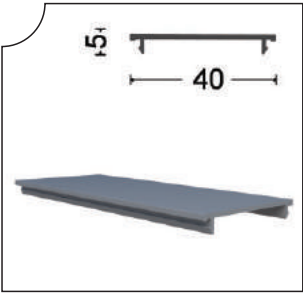
GYTN-1711 Yan Dikme Kapağı Side Cover Profile
