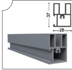
GYTN-1708 Baza 8 mm Profili Aluminum Glass Profile
