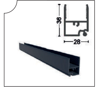
GYTN-1719 Alt-Üst Isıcamlı Baza Bottom-Top Insulating Glass Base
