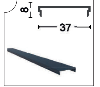
GYTN-1716 Yan Dikme Kapak Side Stand Cover
